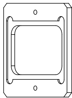
Mirror holder, designed for OLYMPUS 36x25.5mm standard dichroic mirror.
