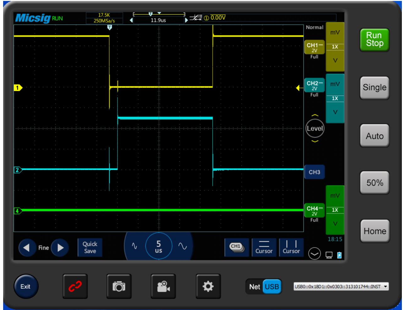
Scope Ch1: TTL out Scope Ch2 Sync out Scope Ch4: Trigger in
